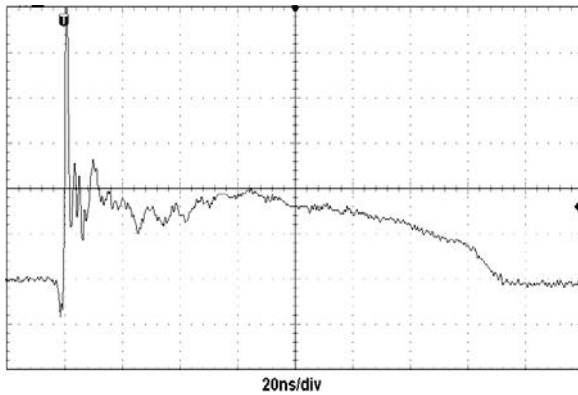
ESD clamping (+8kV contact discharge per IEC61000-4-2)
