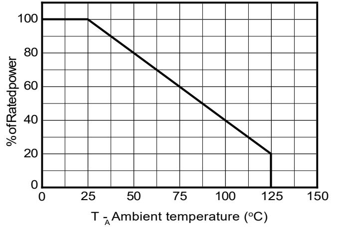
Power derating vs. Ambient temperature
